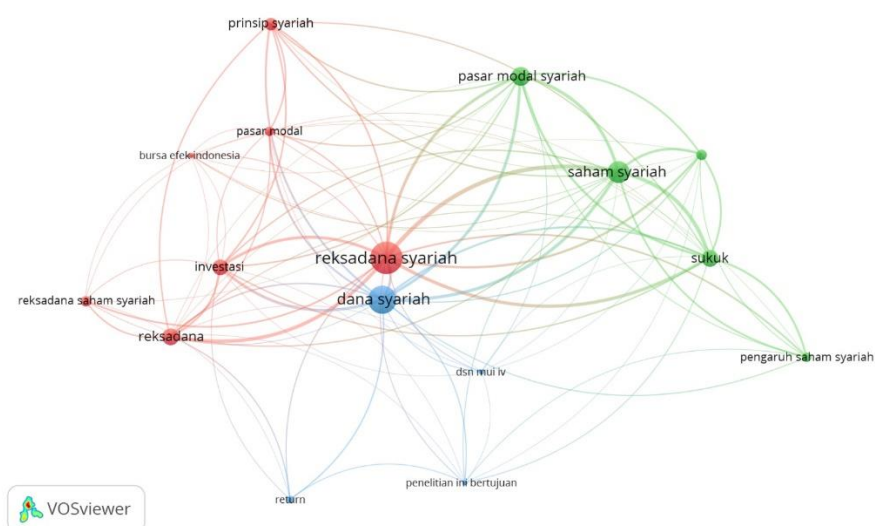
Gambar 1 Network Visualization
