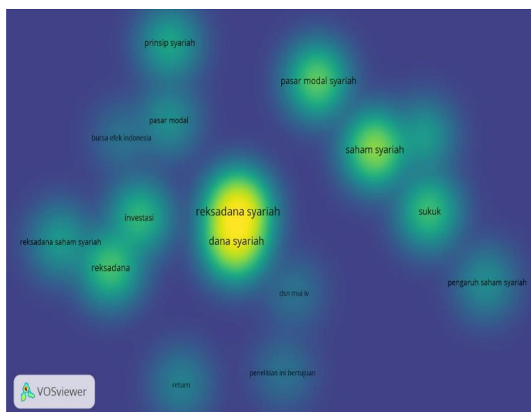
Gambar 3 Density Visualization
